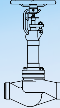
▶ 067 Straight through with butt weld ends
