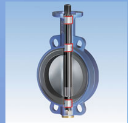
Your cost efficiency: Triple shaft (cylinder liners); operational shaft safety gives long service life
