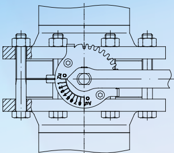
► 014/015 - with lock lever
