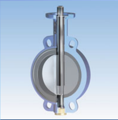
High strength (continuous shaft) provides operational safety
